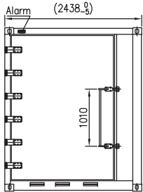
VIEW C
