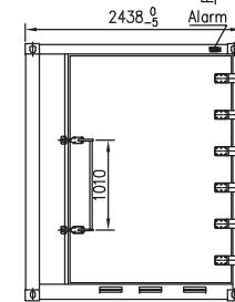
VIEW E
