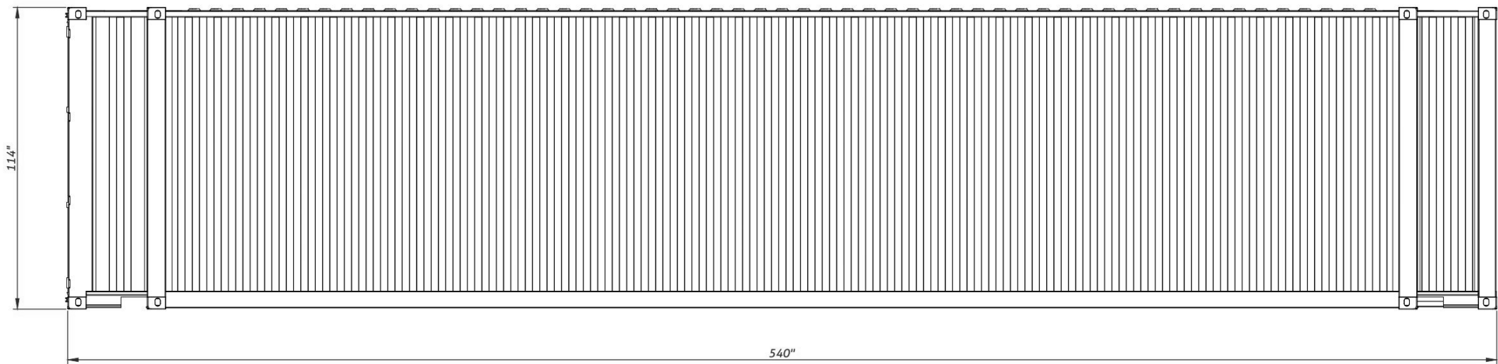
● Right view
